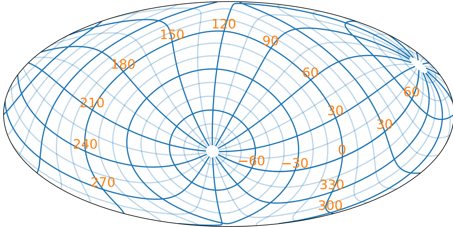
Hammer projection in ICRS coordinates with the corresponding Galactic grid overlaid
